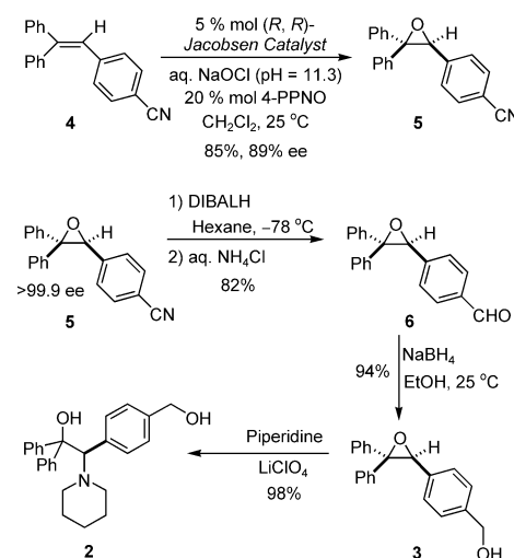
Scheme 2. Synthesis of ligand 2 .
