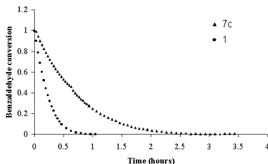
Figure 3. Profiles of benzaldehyde conversion for the addition of diethylzinc to benzaldehyde mediated by resin 7c and the homogeneous phase ligand 1 .
