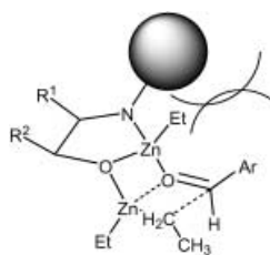
Figure 4. Perturbation of the active site by the polymeric matrix in amino alcohol ligands anchored through the nitrogen atom.
