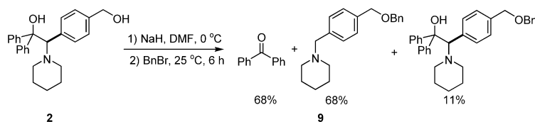
Scheme 4. Fragmentation of ligand 2 under basic conditions.
