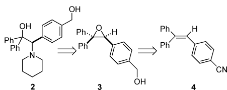
Scheme 1. Retrosynthetic strategy for the preparation of ligand 2 .
