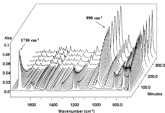
Figure 1. FTIR absorbance spectra during the addition of diethylzinc to benzaldehyde mediated by resin 7a .
