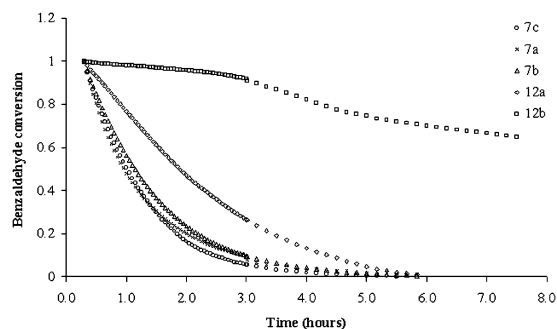
Figure 2. Profiles of benzaldehyde conversion for the addition of diethylzinc to benzaldehyde mediated by resin 7a–c and 12a, b .
